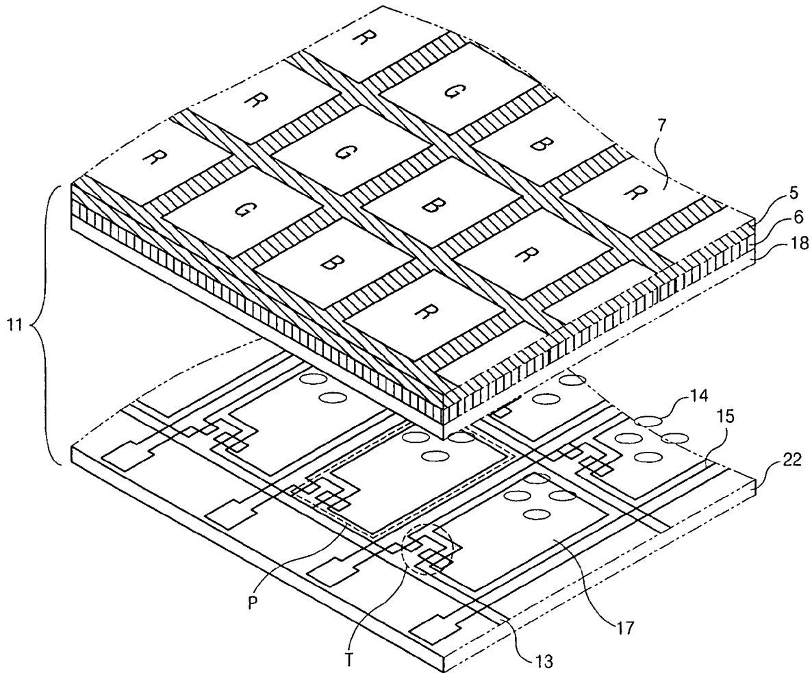
FIG. 1 (RELATED ART)
